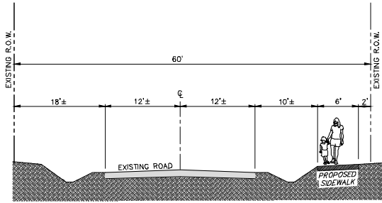
TYPICAL SIDEWALK SECTION - 60' R.O.W. A.T.S.
